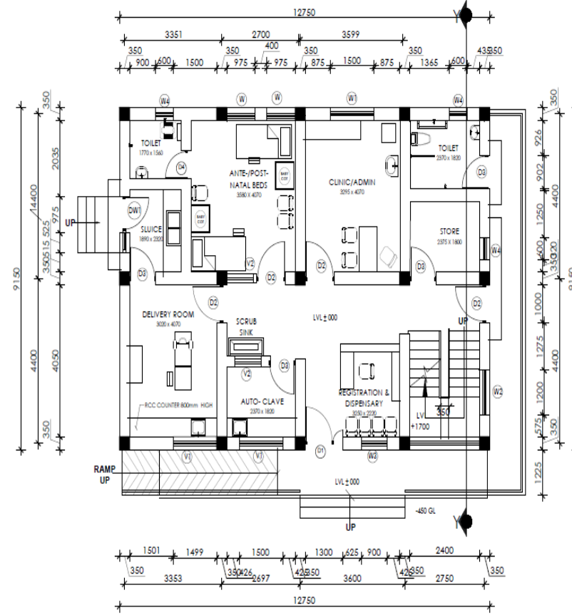
GROUND FLOOR PLAN AREA: 145.36 SQ. M.
